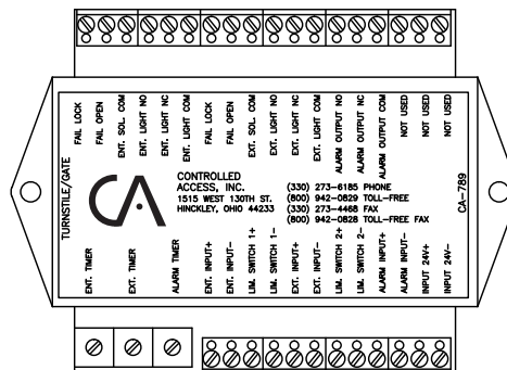
Control Board 0789
